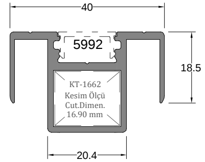
Cam - Panel Kanat Profil GLASS - PANEL SASH PROFILE
